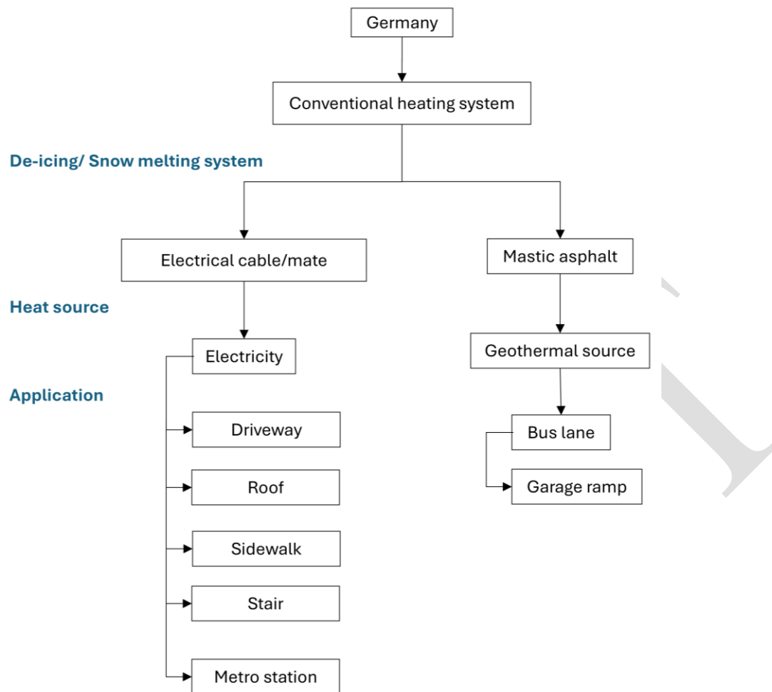
Figure 3. General mapping of de-icing and snow-melting applications in Germany utilizing non-hydronic heating system, and the corresponding heat sources.
