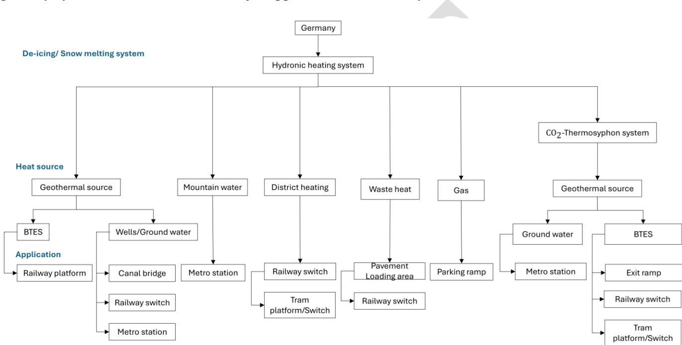
Figure 2. General mapping of de-icing and snow-melting applications in Germany utilizing hydronic heating system, and the corresponding heat sources.
